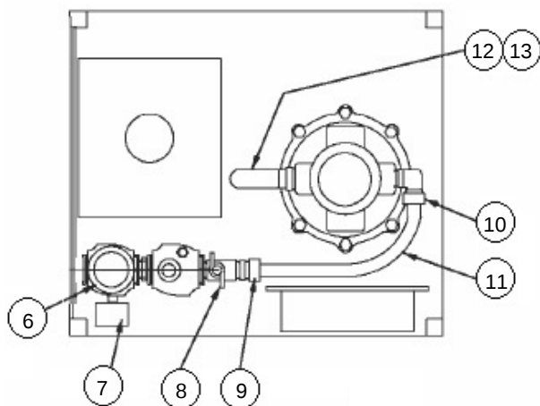
LAYOUT OF PNEUMATIC PIPWORK
