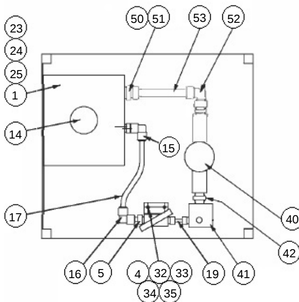
LAYOUT OF HYDRAULIC PIPEWORK
