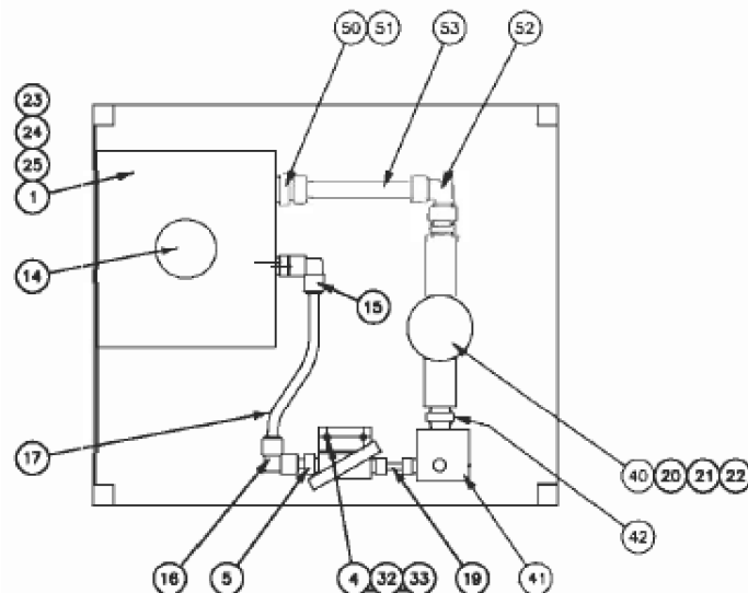
LAYOUT OF HYDRAULIC PIPEWORK
