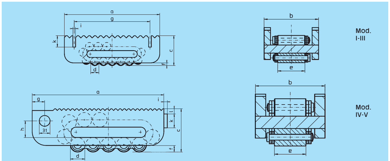
Picture showing hardened steel chain rollers
